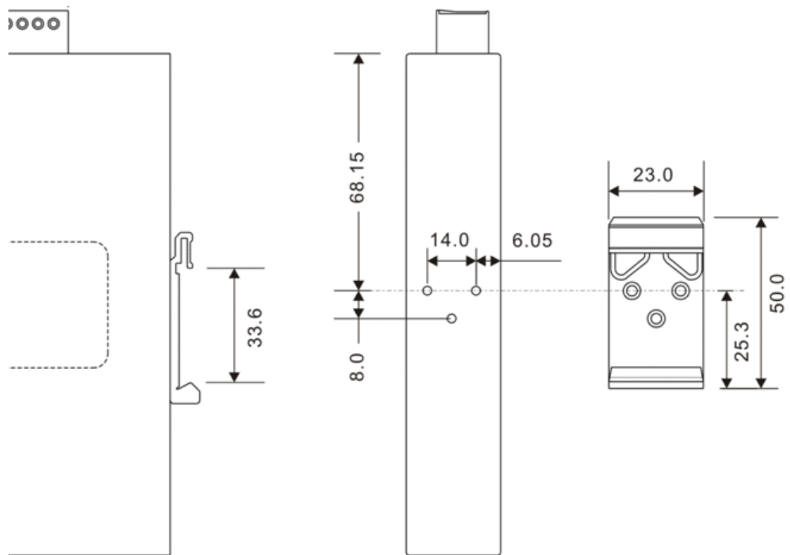
DIN-Rail Size
